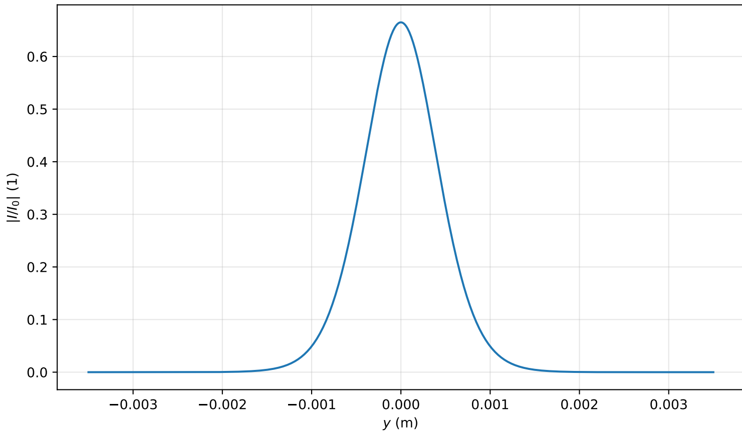
Intensity profile I(x=0, y, z=2.229)/I_0 , P_{in}=0.4P_{cr} , artificial time
